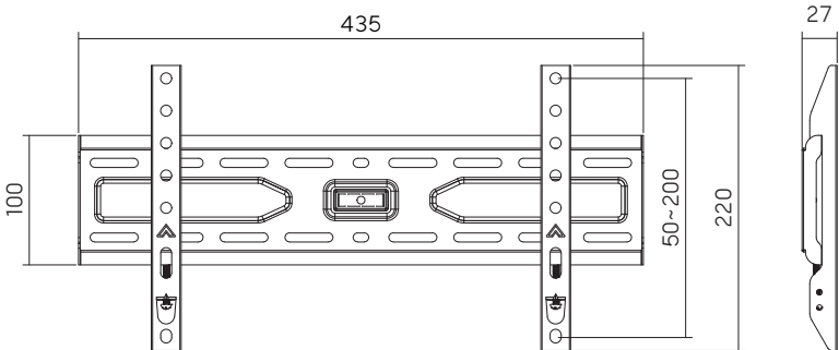
Dimensions(mm)
